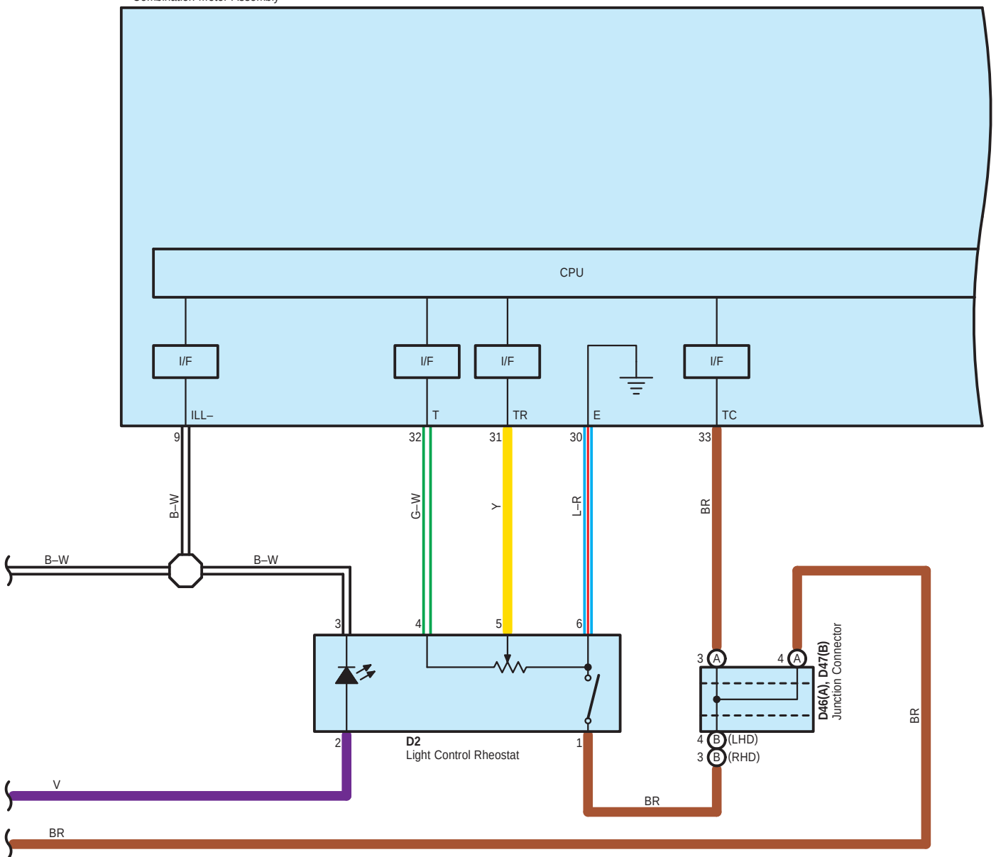
D7 Combination Meter Assembly
