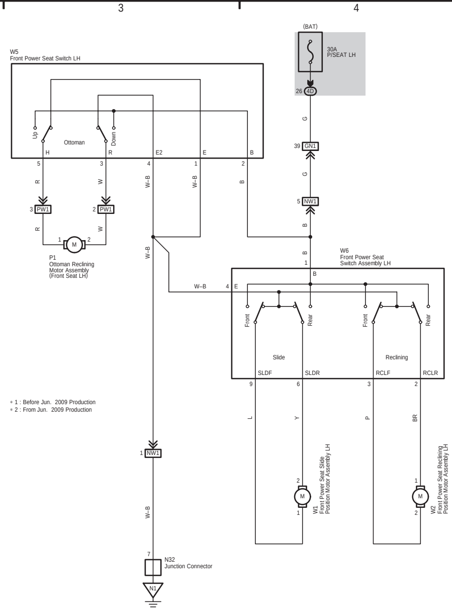
Power Seat (RHD Front Passenger' s Seat) (Before Oct. 2011 Production)
