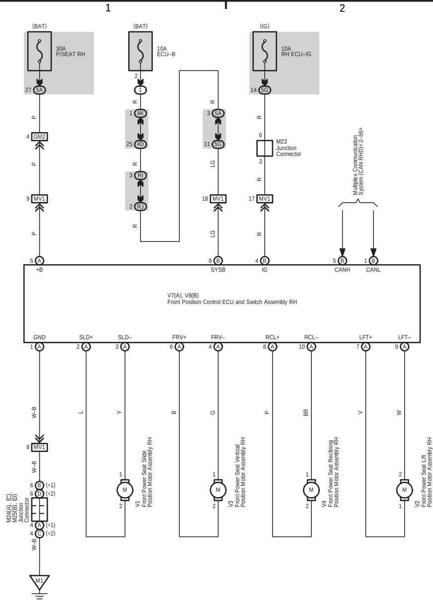
Power Seat (RHD Driver' s Seat) (Before Oct. 2011 Production)
