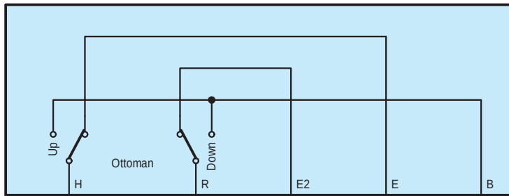
V10 Front Power Seat Switch RH
