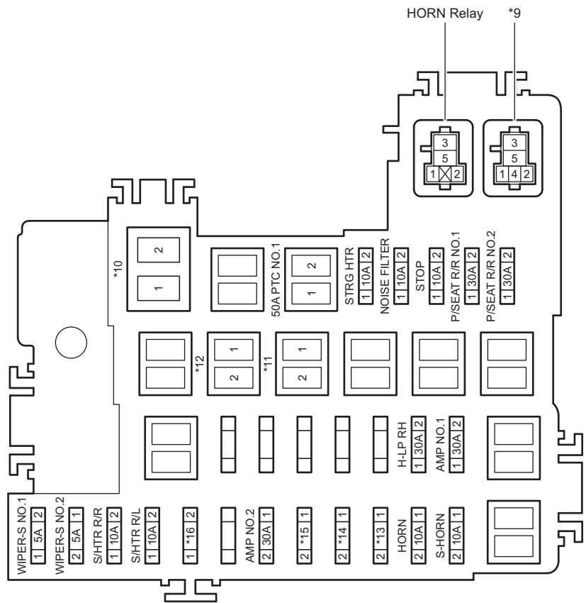
Top View
