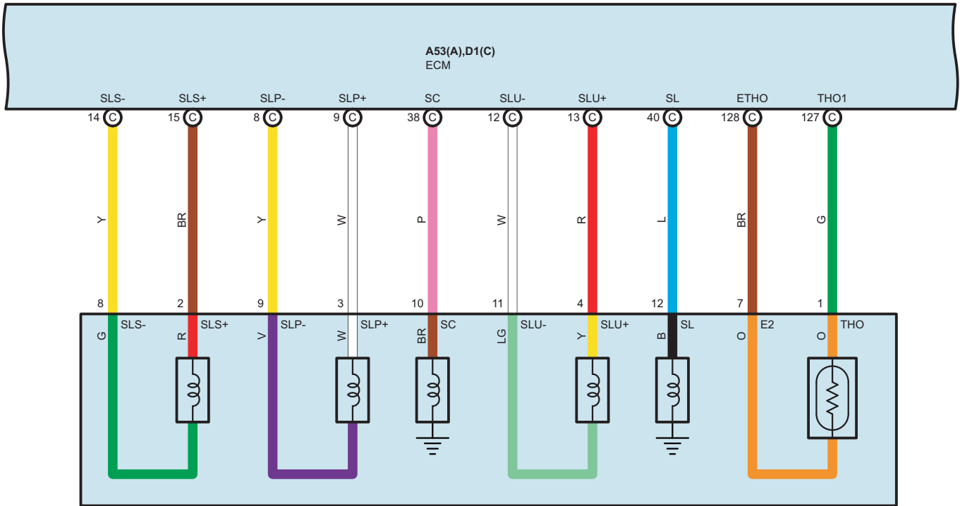
D35 Electronic Control Transmission Solenoid (Transmission Wire)
