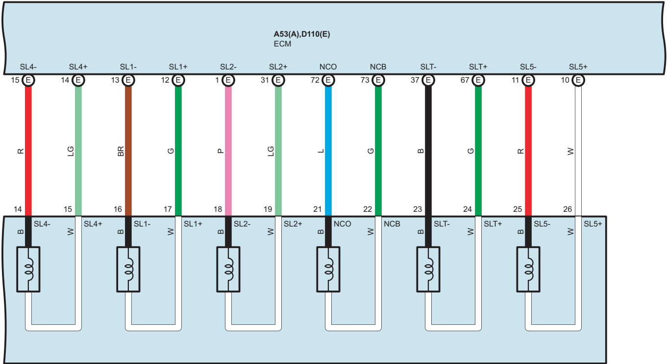
D75 Electronic Control Transmission Solenoid (Transmission Wire)
