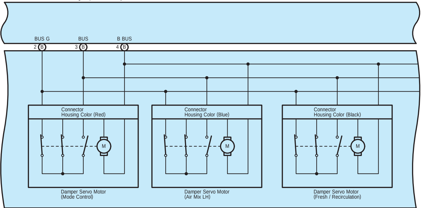
z3(B) Air Conditioning Blower Assembly
