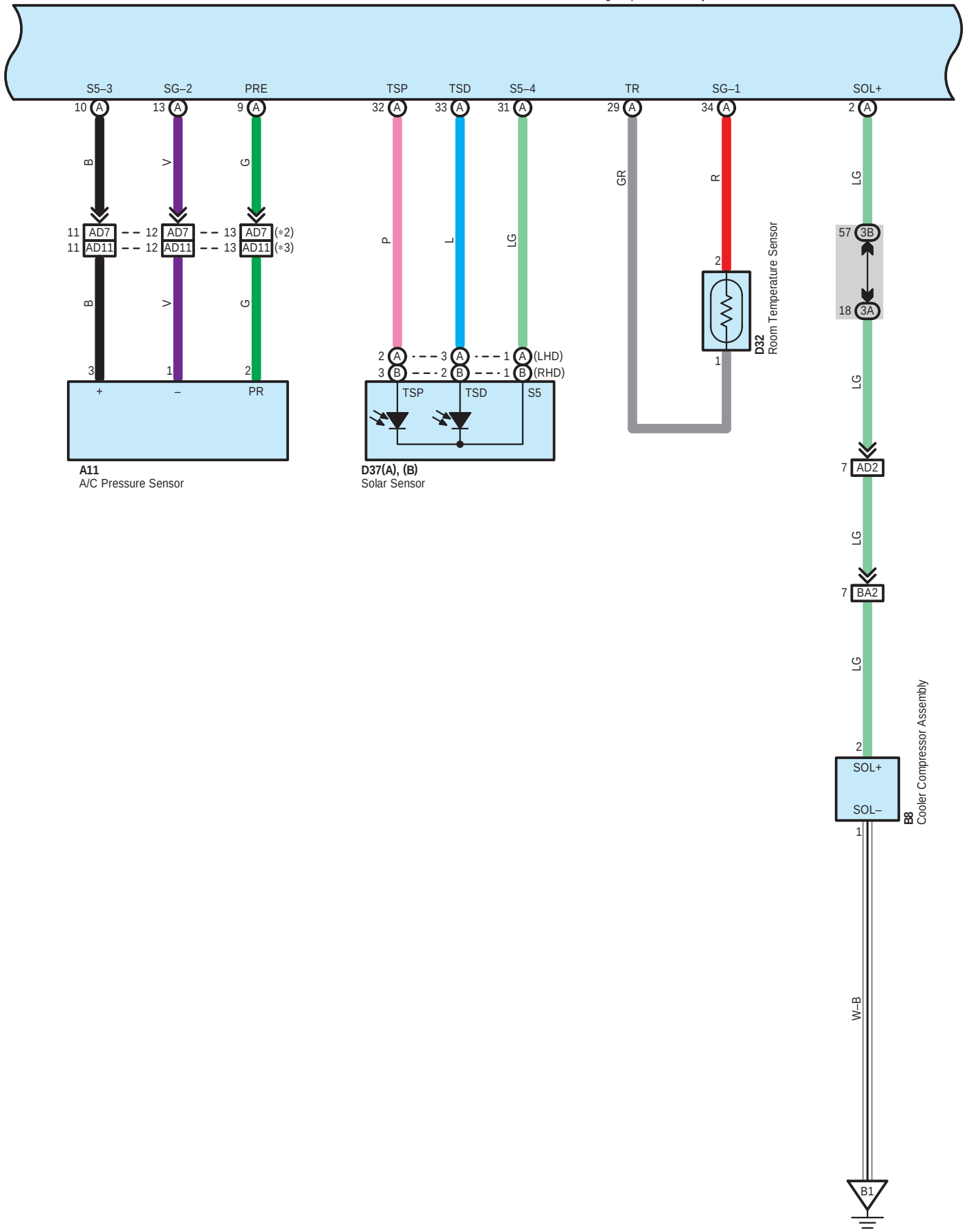
D47(A), z3(B) Air Conditioning Amplifier Assembly
