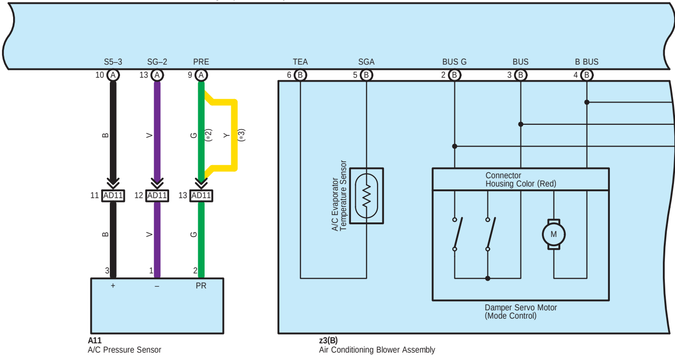
D101(A), z3(B) Air Conditioning Amplifier Assembly
