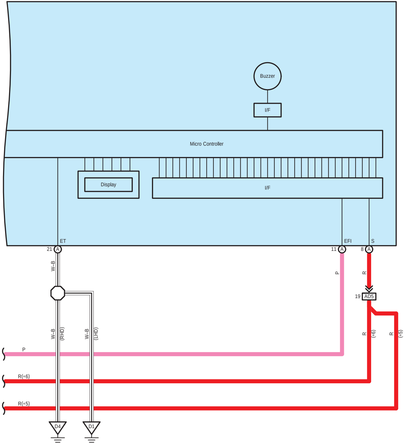
D66(A) Combination Meter
