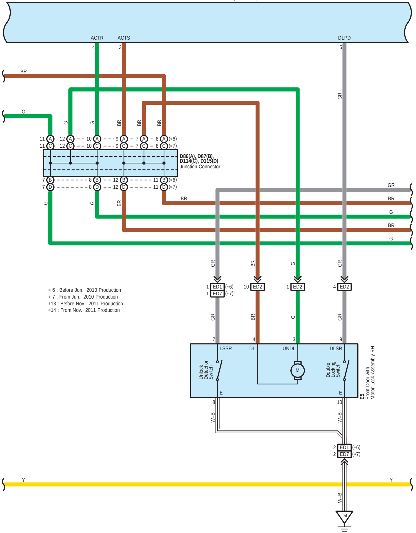
D107 Double Lock Door Control Relay Assembly
