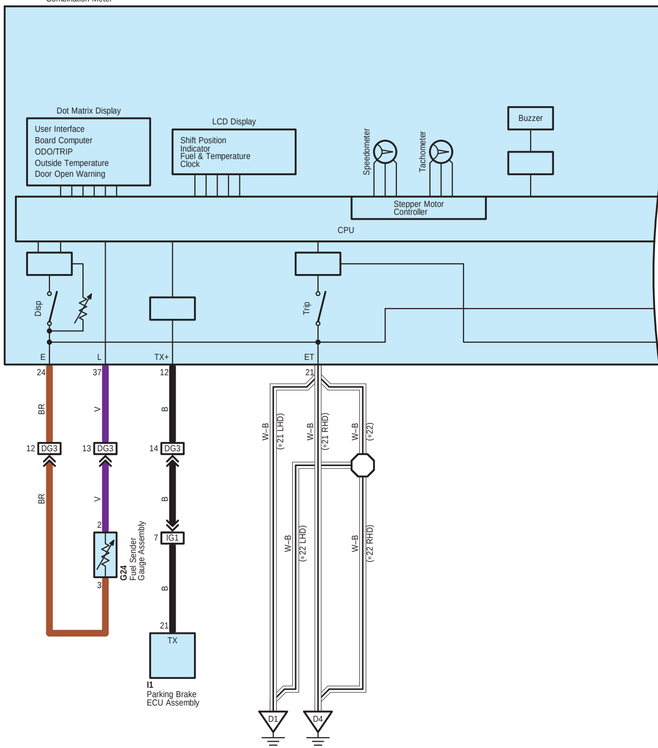
D66 Combination Meter
