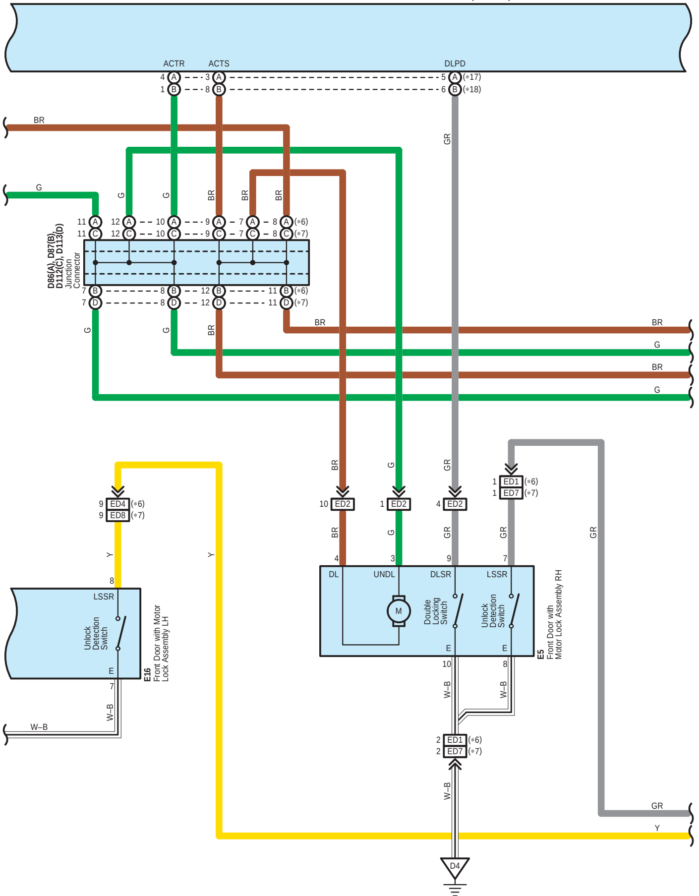
D107(A), D162(B) Double Lock Door Control Relay Assembly
