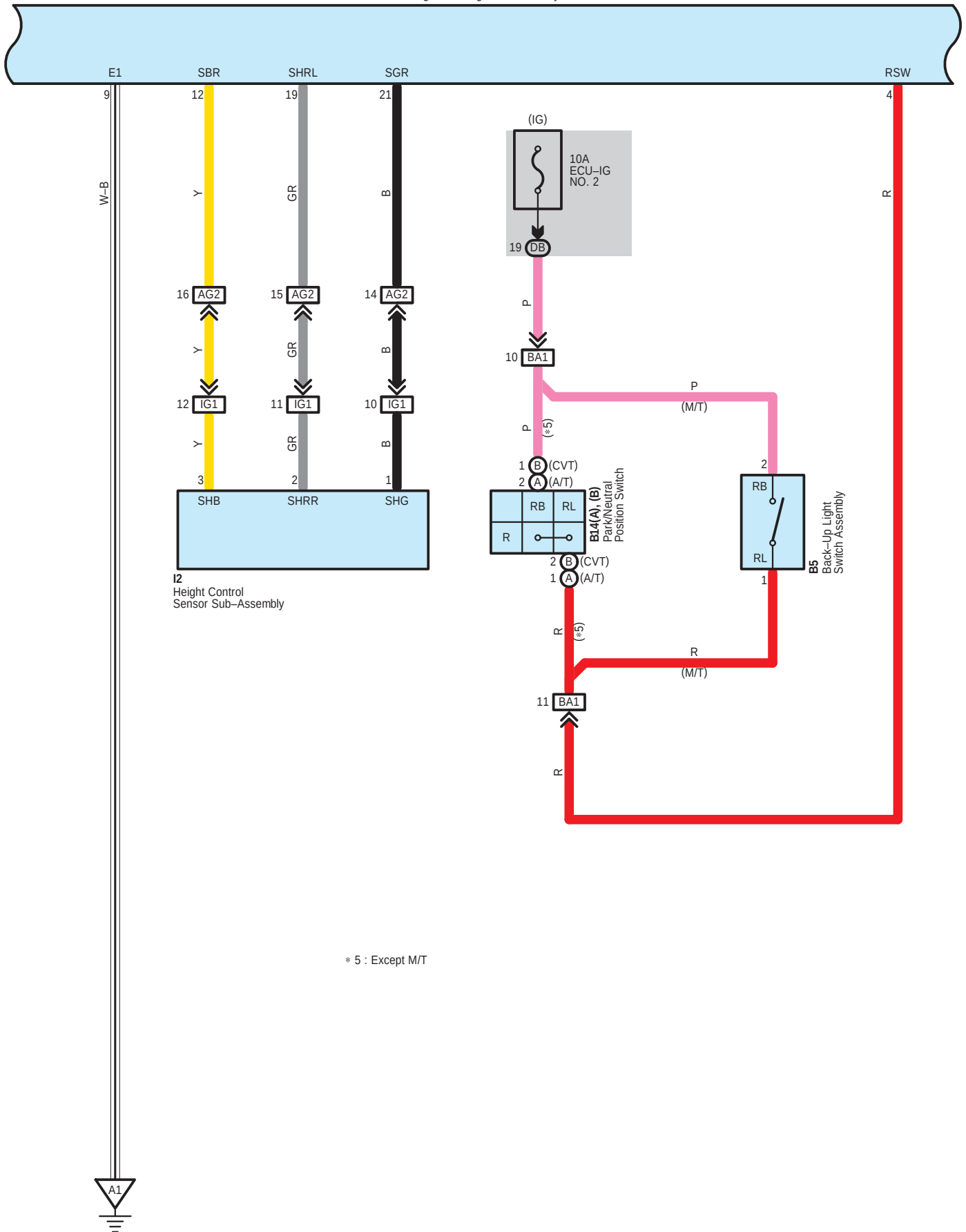
A66 Headlight Leveling ECU Assembly
