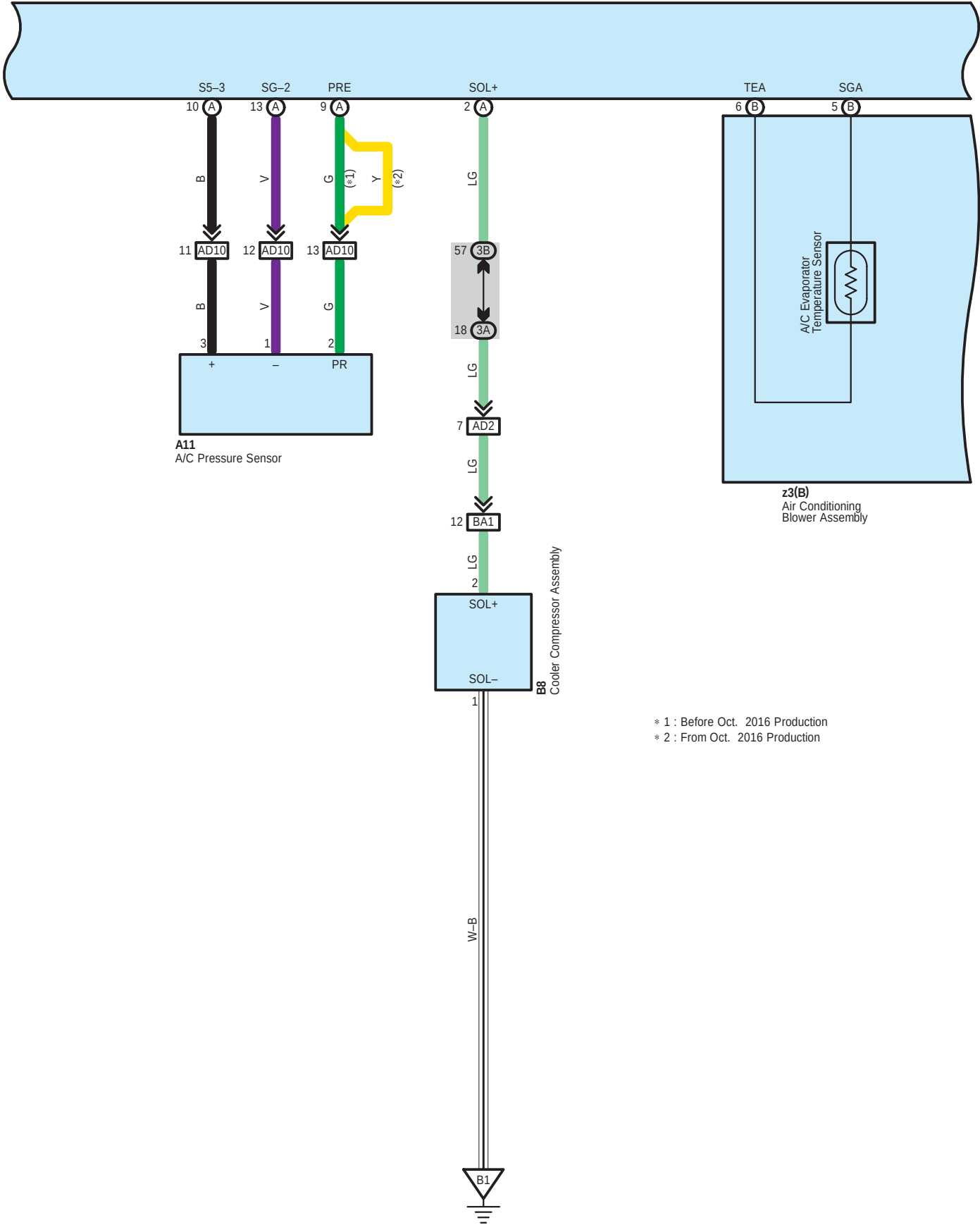
D101(A), z3(B) Air Conditioning Amplifier Assembly
