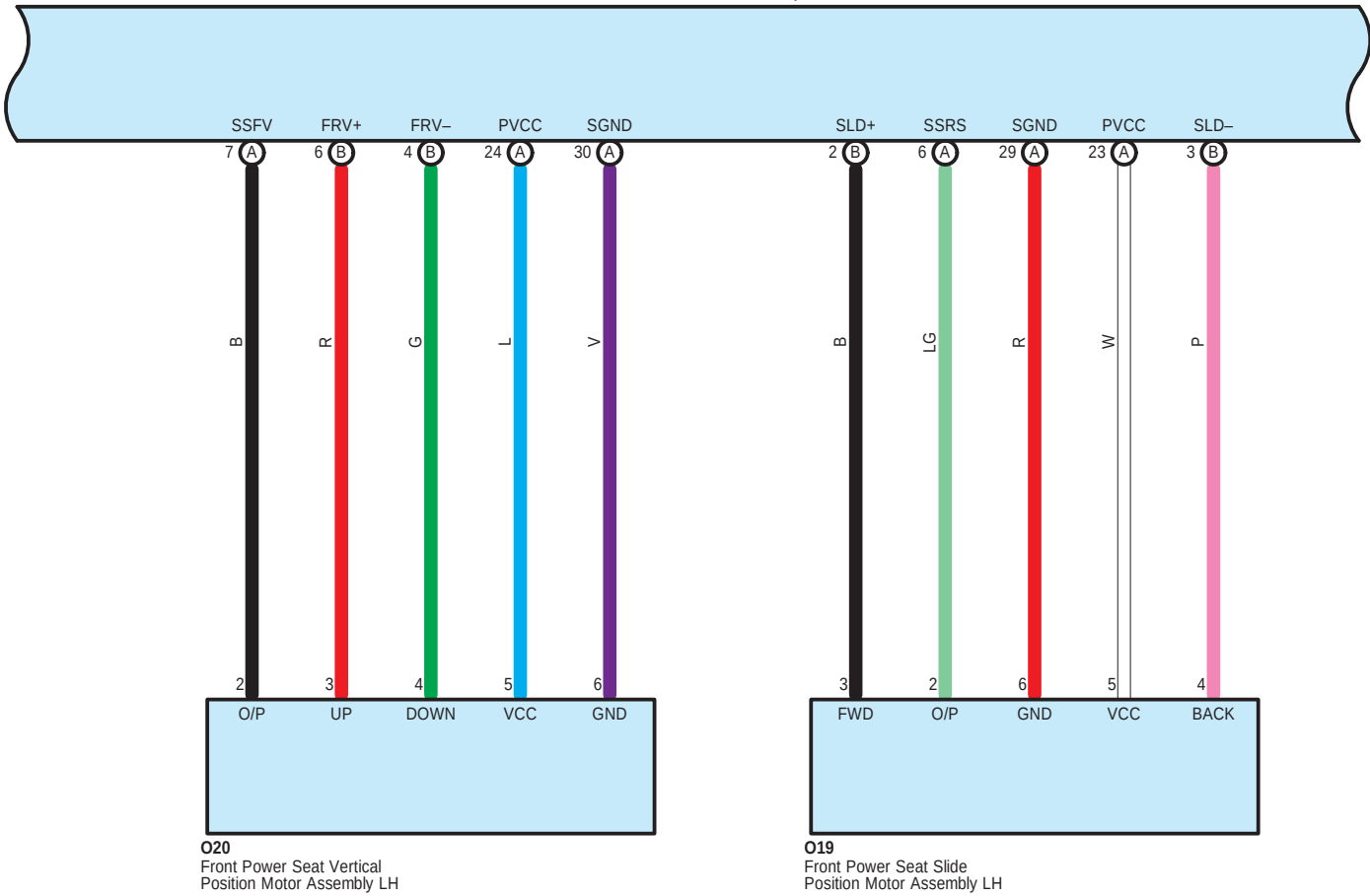
O26(A), O27(B) Position Control ECU Assembly
