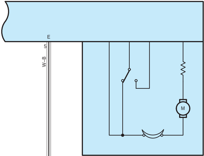
M1 Rear Wiper Motor Assembly
