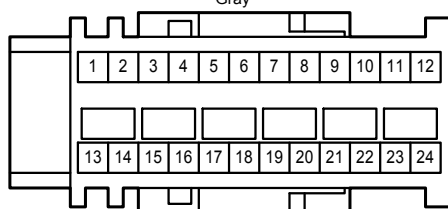
H 25
