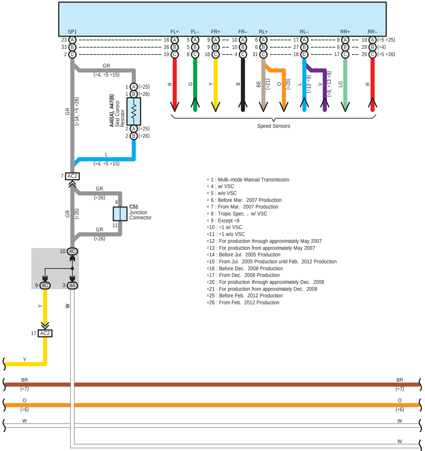
A21(A), A41(B), A46(C) Skid Control ECU with Actuator
