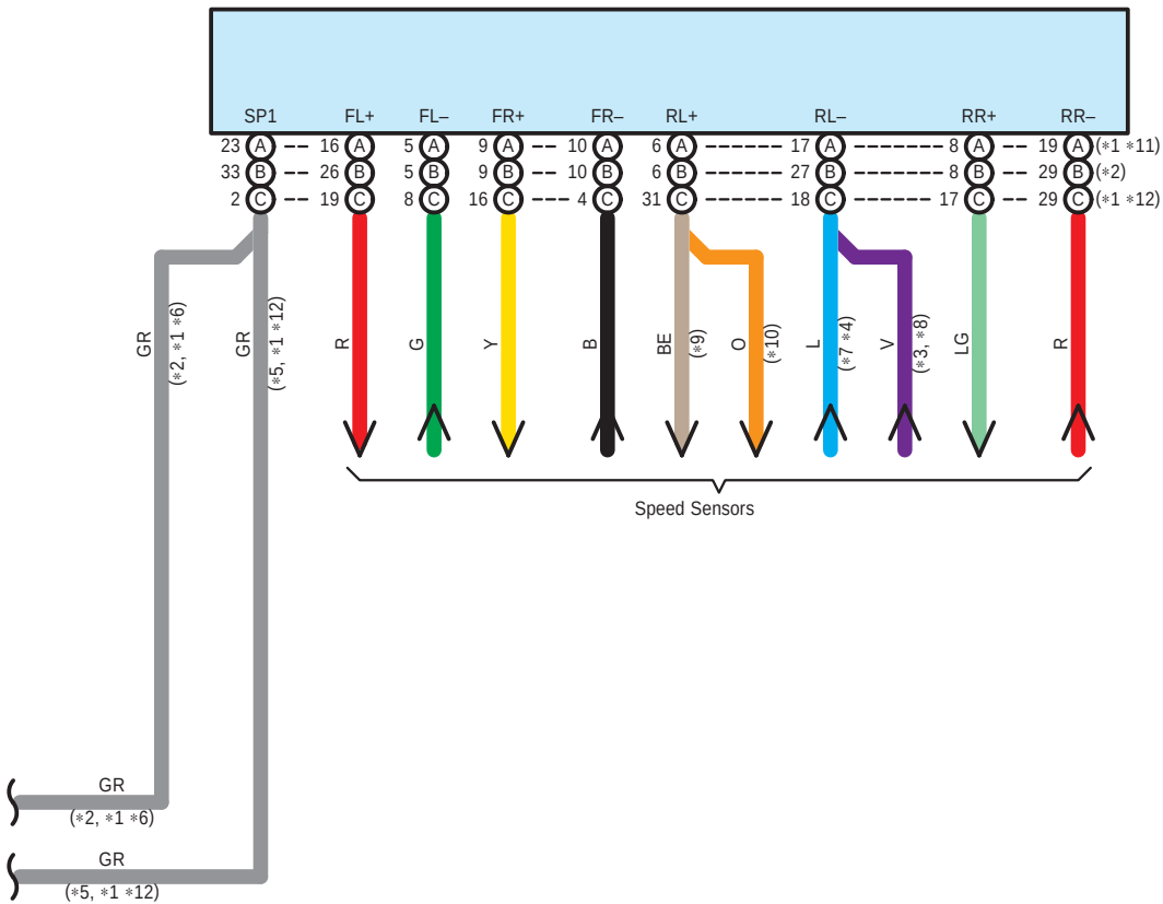
A21(A), A41(B), A46(C) Skid Control ECU with Actuator
