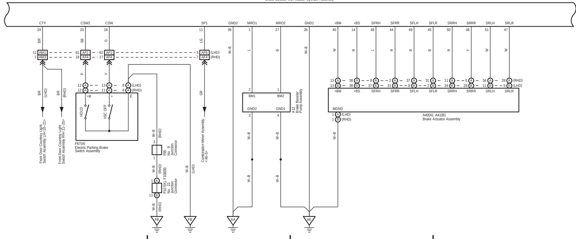
A39 Brake Booster with Master Cylinder Assembly
