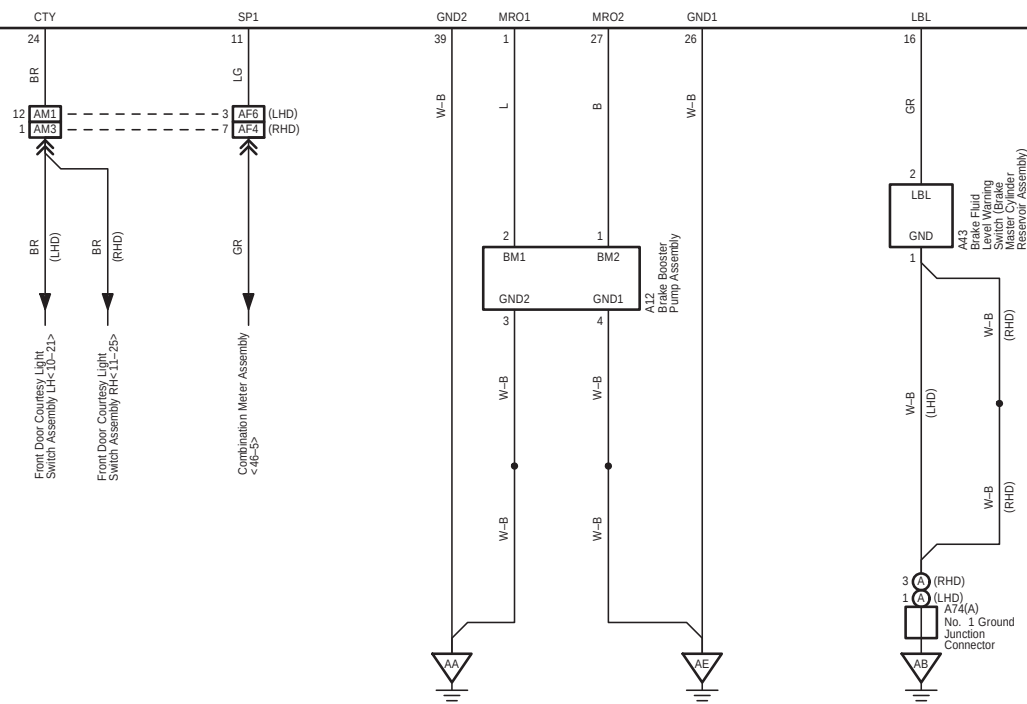
A39 Brake Booster with Master Cylinder Assembly
