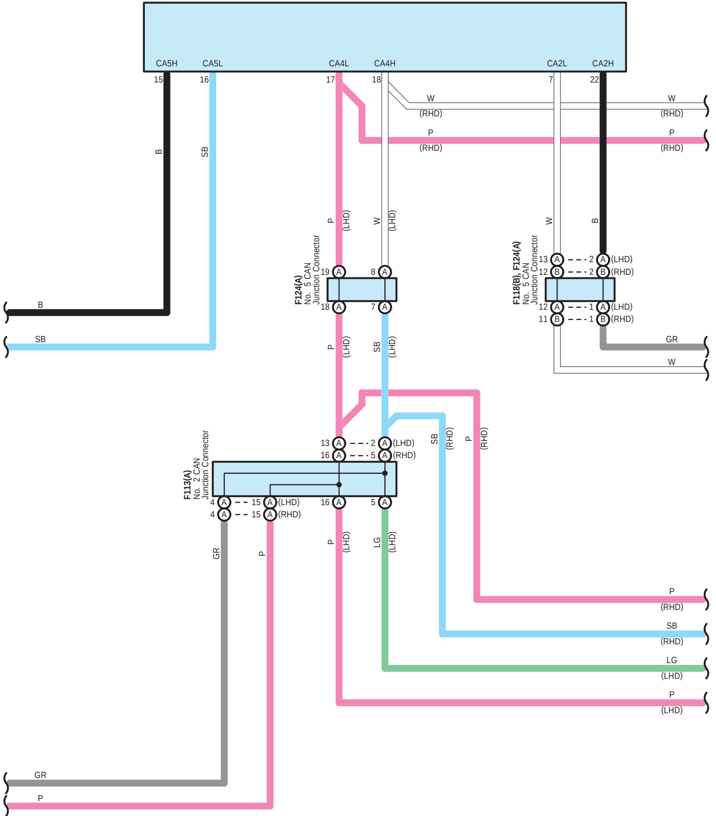
F74 Network Gateway ECU
