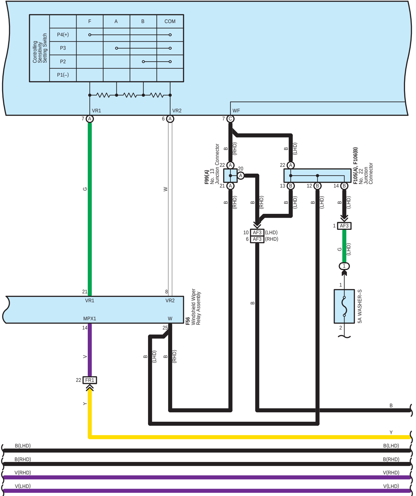
F26(A), F36(C) Windshield Wiper Switch Assembly
