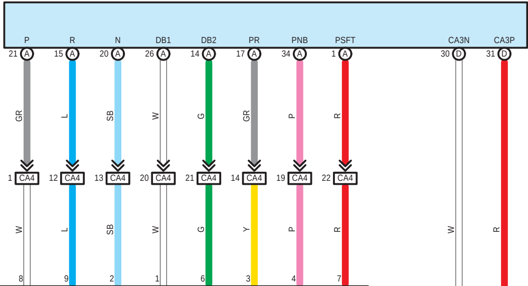
A48(A), F3(D) Hybrid Vehicle Control ECU
