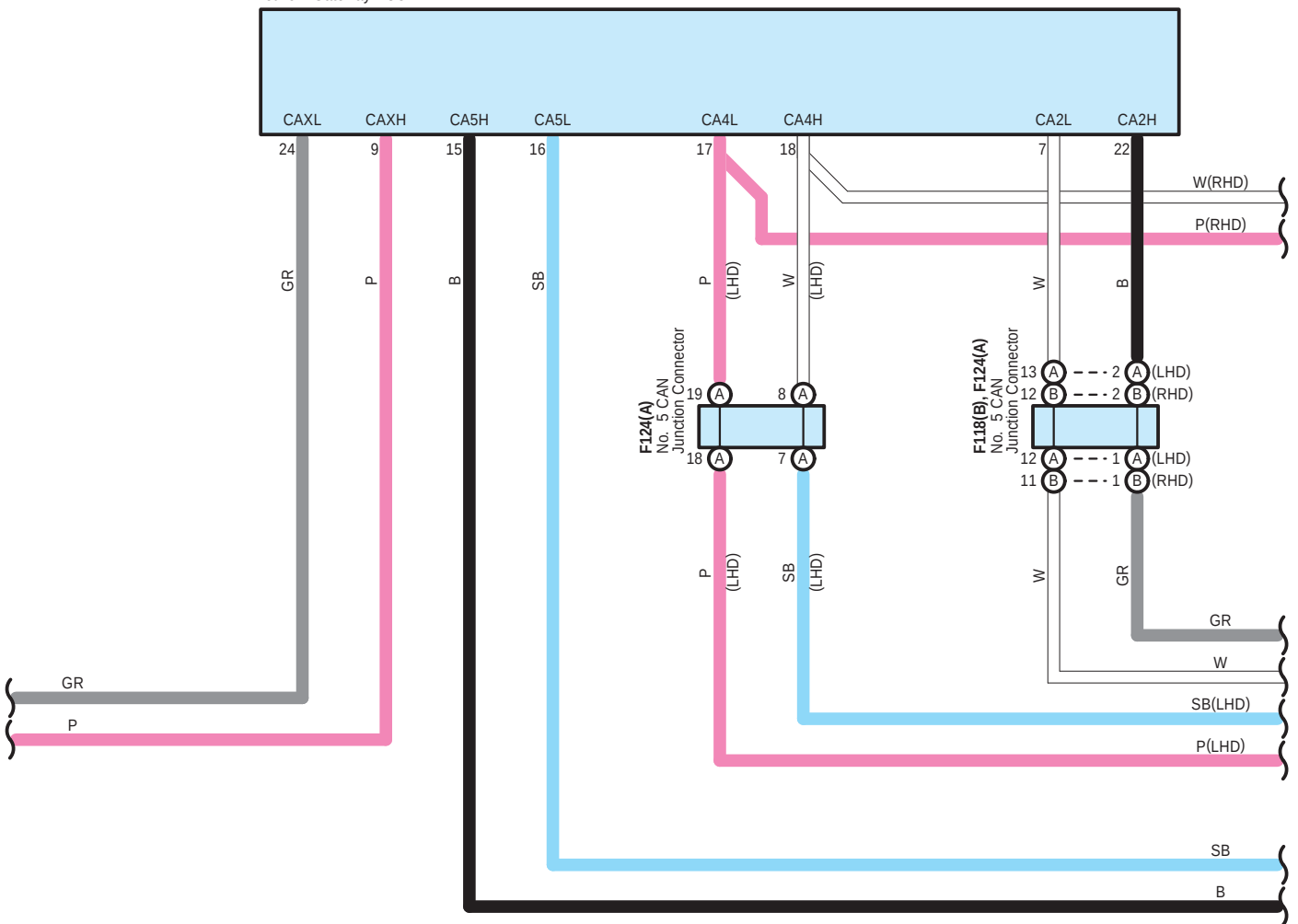
F74 Network Gateway ECU
