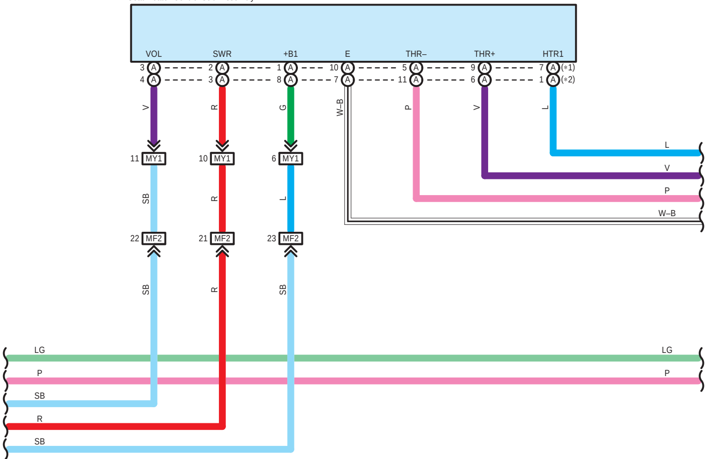
Y4(A) Seat Heater Control Sub-Assembly RH
