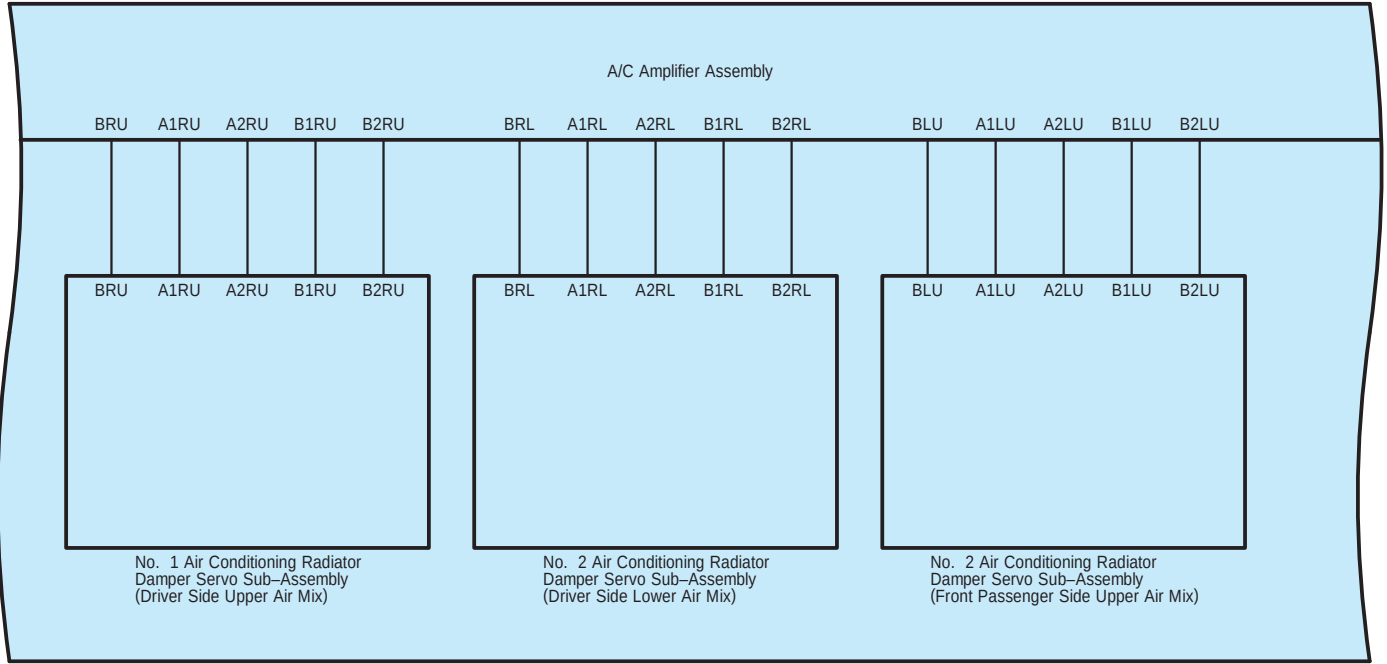
A83(C), F8(A), F72(B) A/C Unit Assembly
