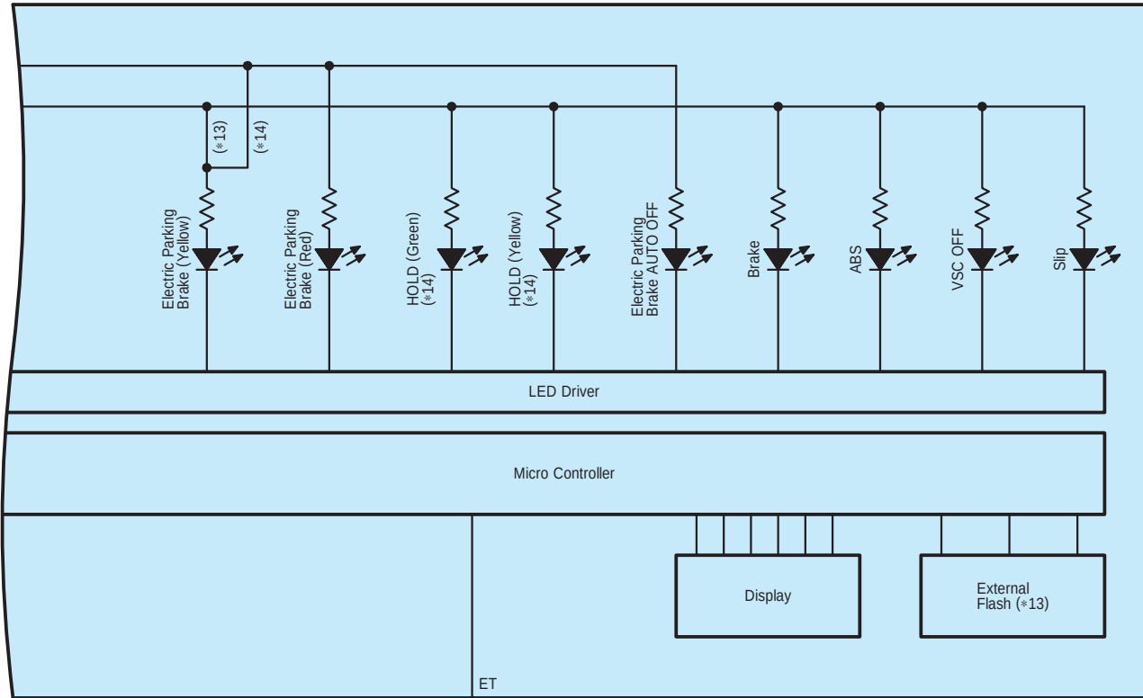
F4(A) Combination Meter Assembly
