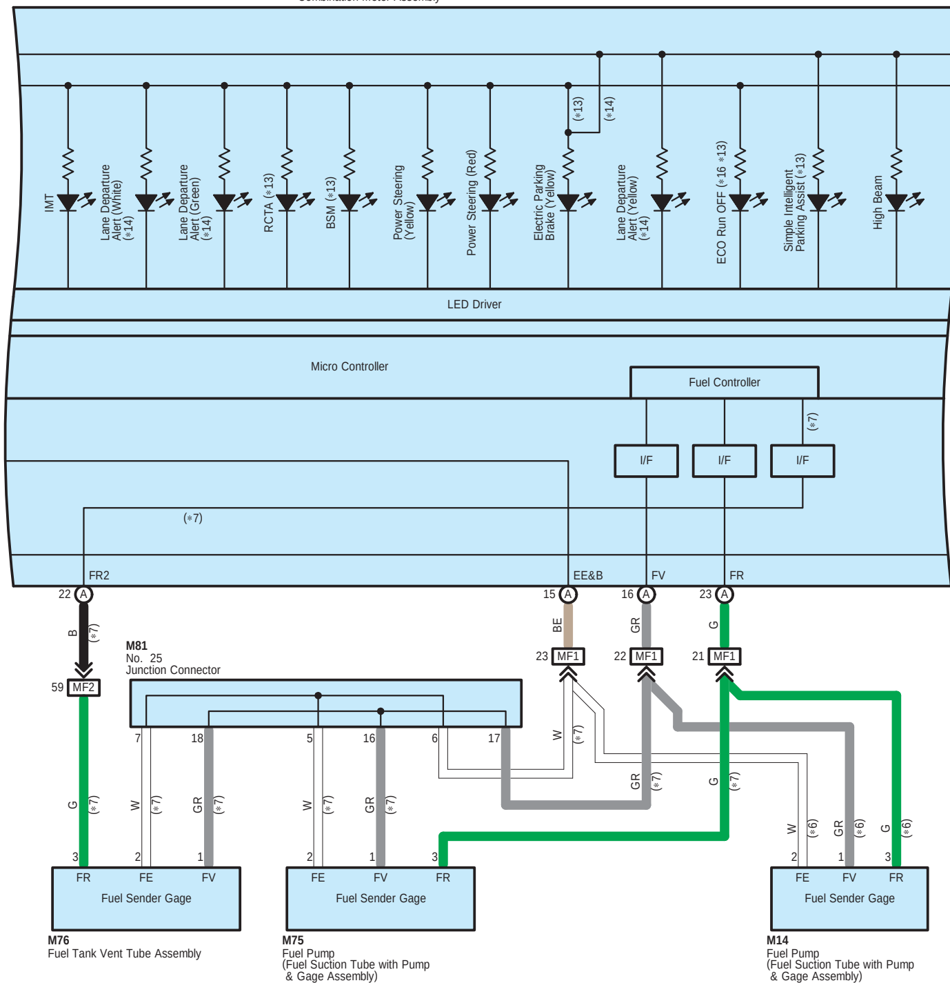
F4(A), F5(B) Combination Meter Assembly
