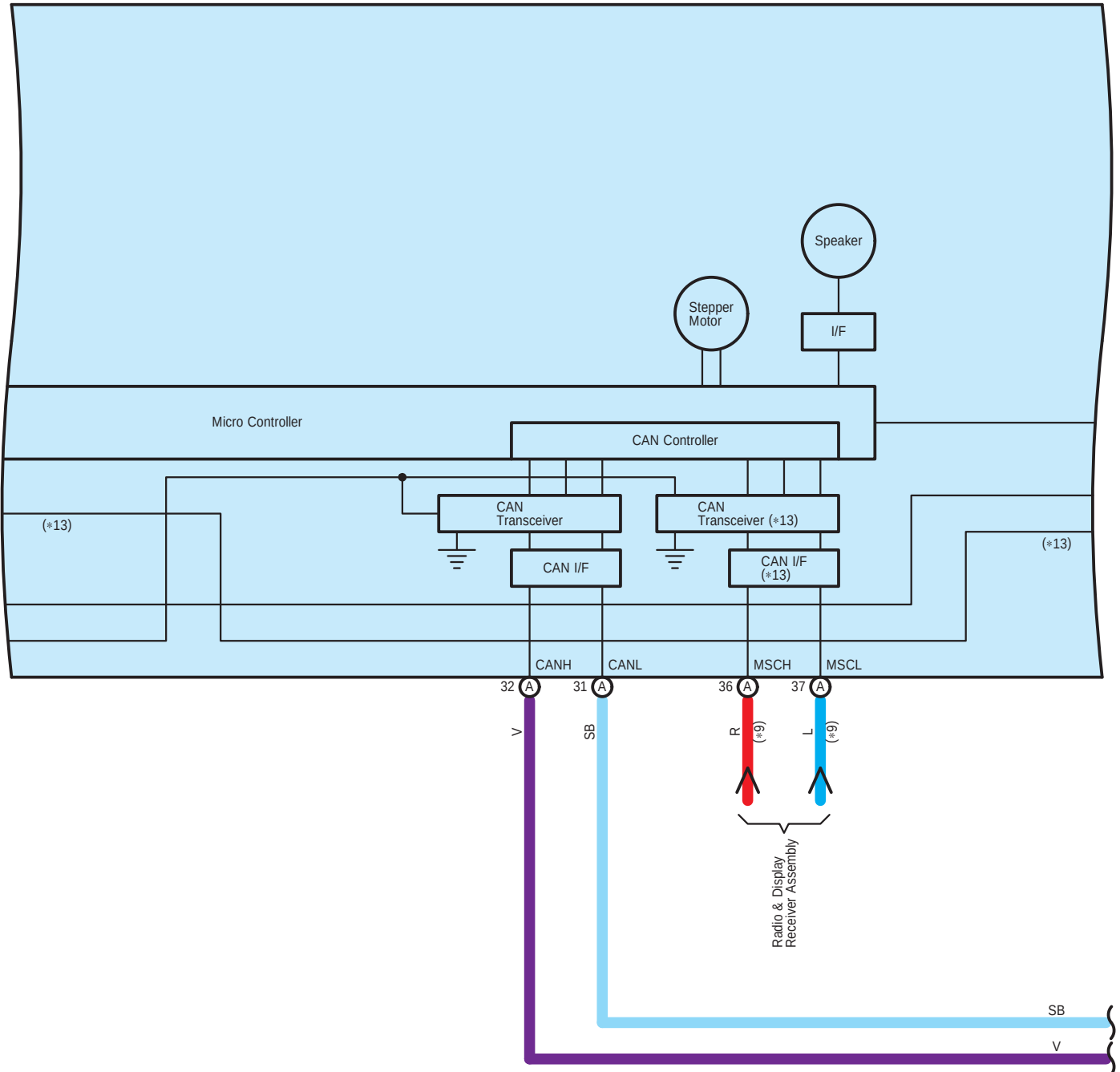
F4(A), F5(B) Combination Meter Assembly
