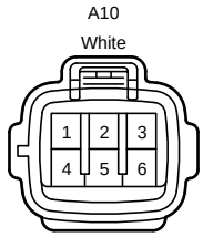
90980-11194 (Halogen Headlight Type)
