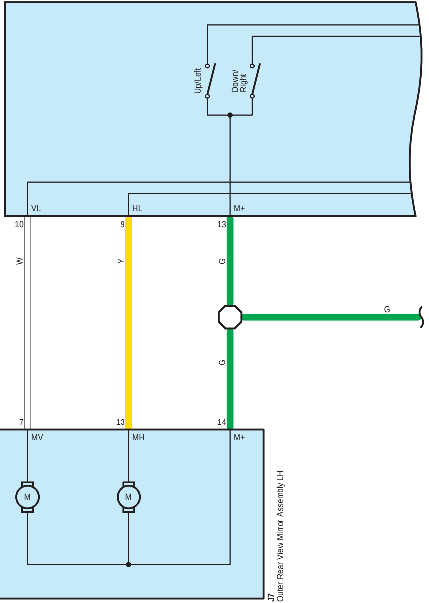
J10 Outer Mirror Switch Assembly
