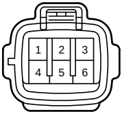
90980-11194 (Clearance, DRL, High, Turn)
