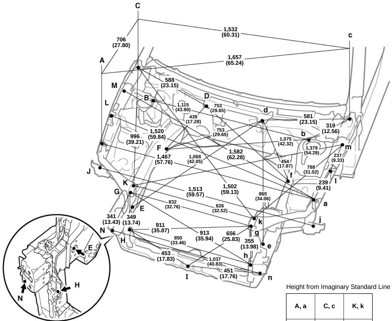
Vehicle Dimensions
