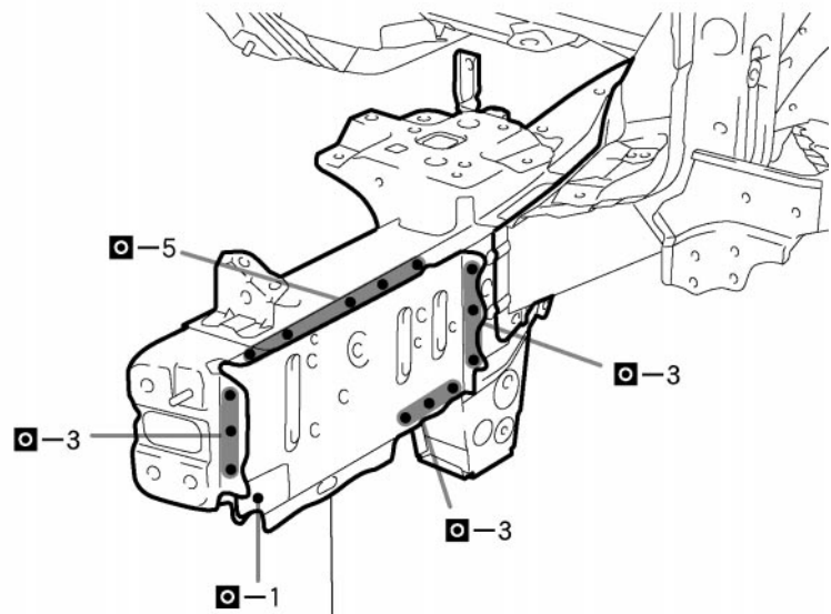
Front Side Member Extension
