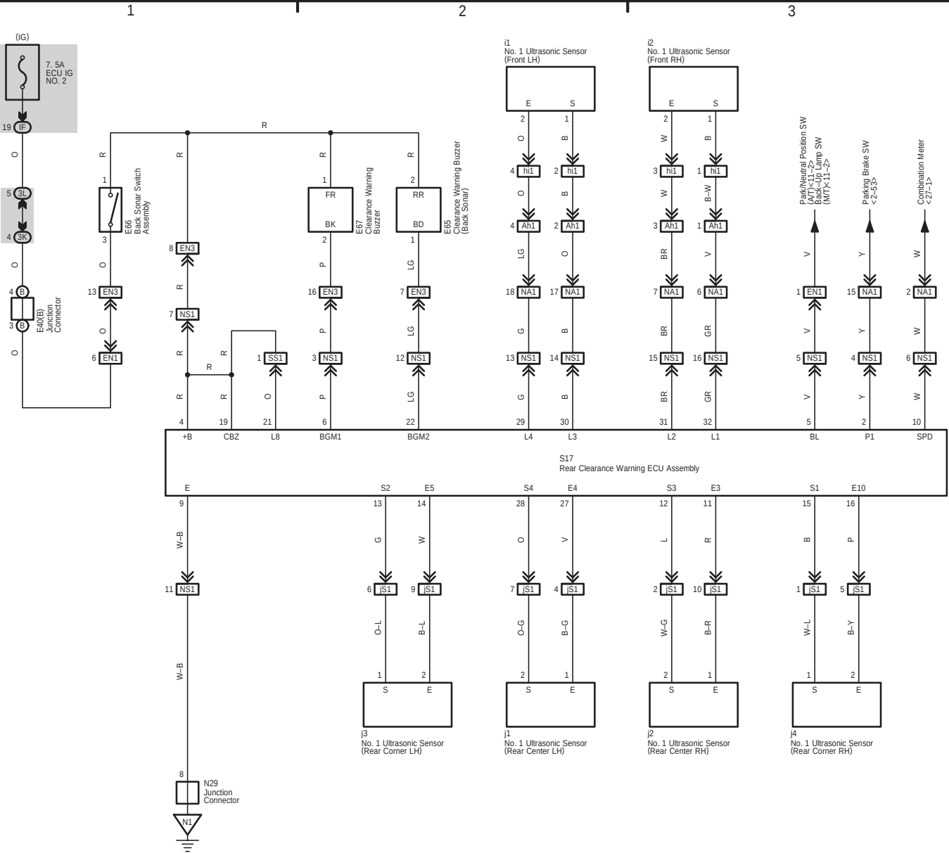
Parking Assist (TOYOTA Parking Assist–Sensor) (Before Jan. 2009 Production)
