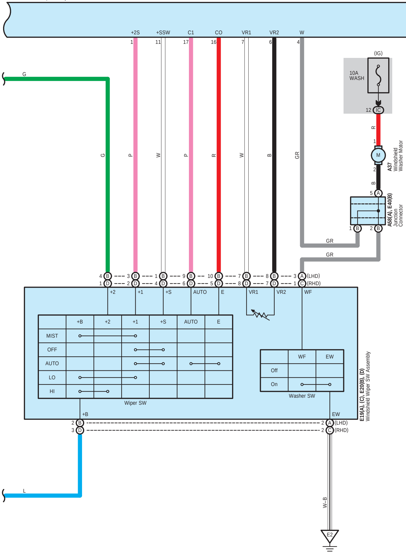
E26 Windshield Wiper Relay
