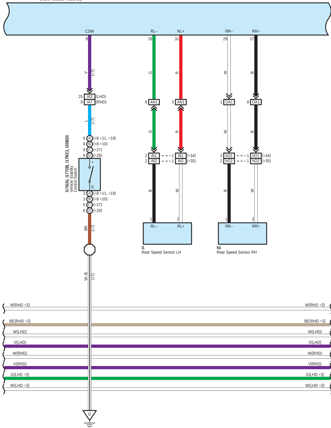
A49 Brake Actuator Assembly
