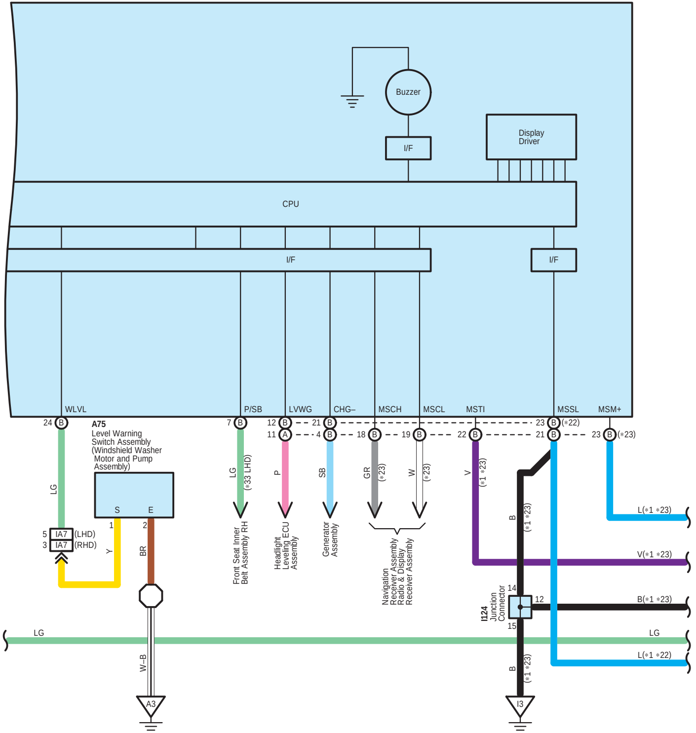
I17(A), I18(B) Combination Meter Assembly
