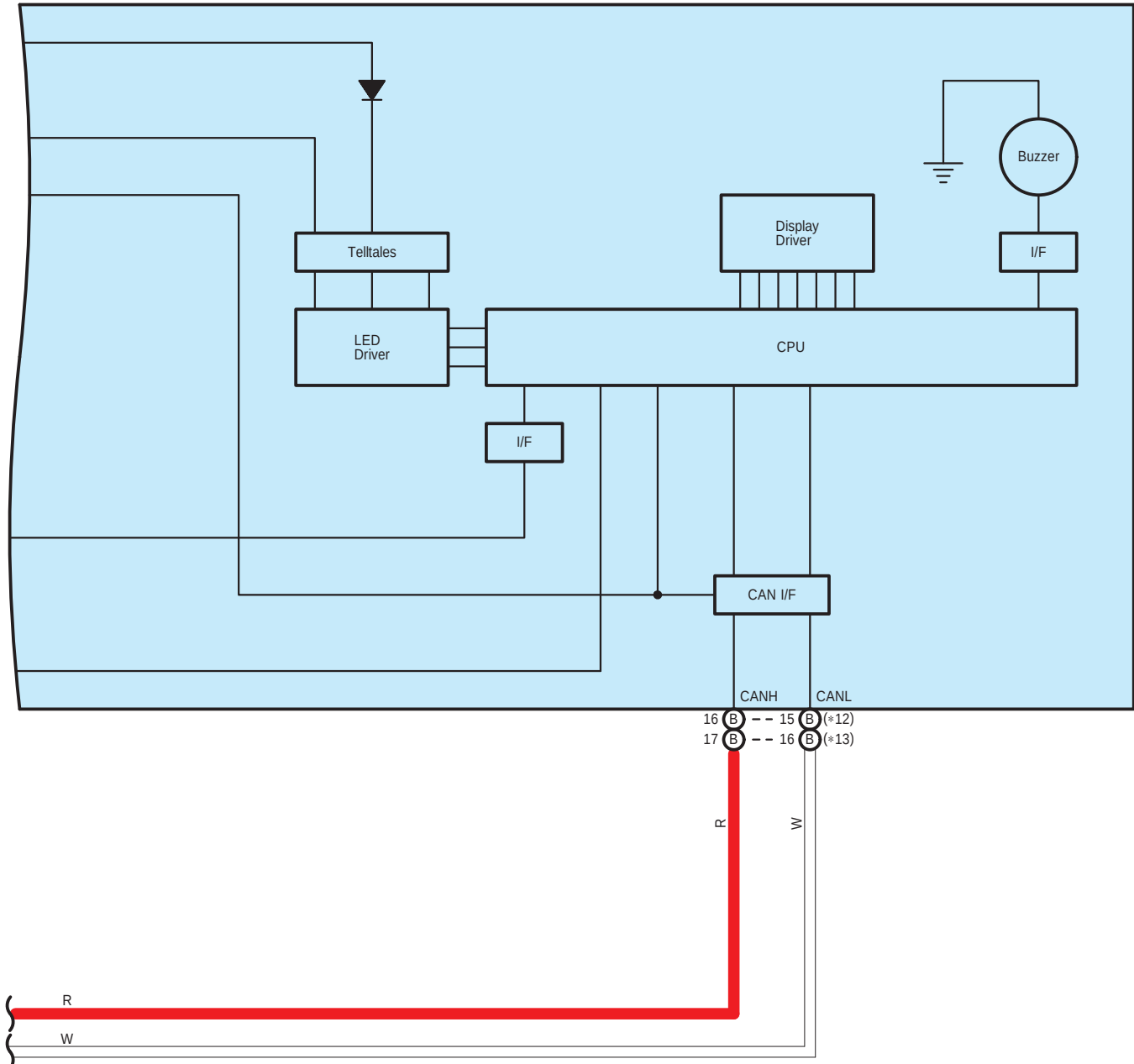
I17(A), I18(B) Combination Meter Assembly
