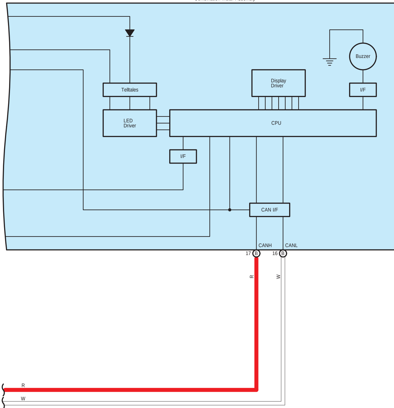
I17(A), I18(B) Combination Meter Assembly
