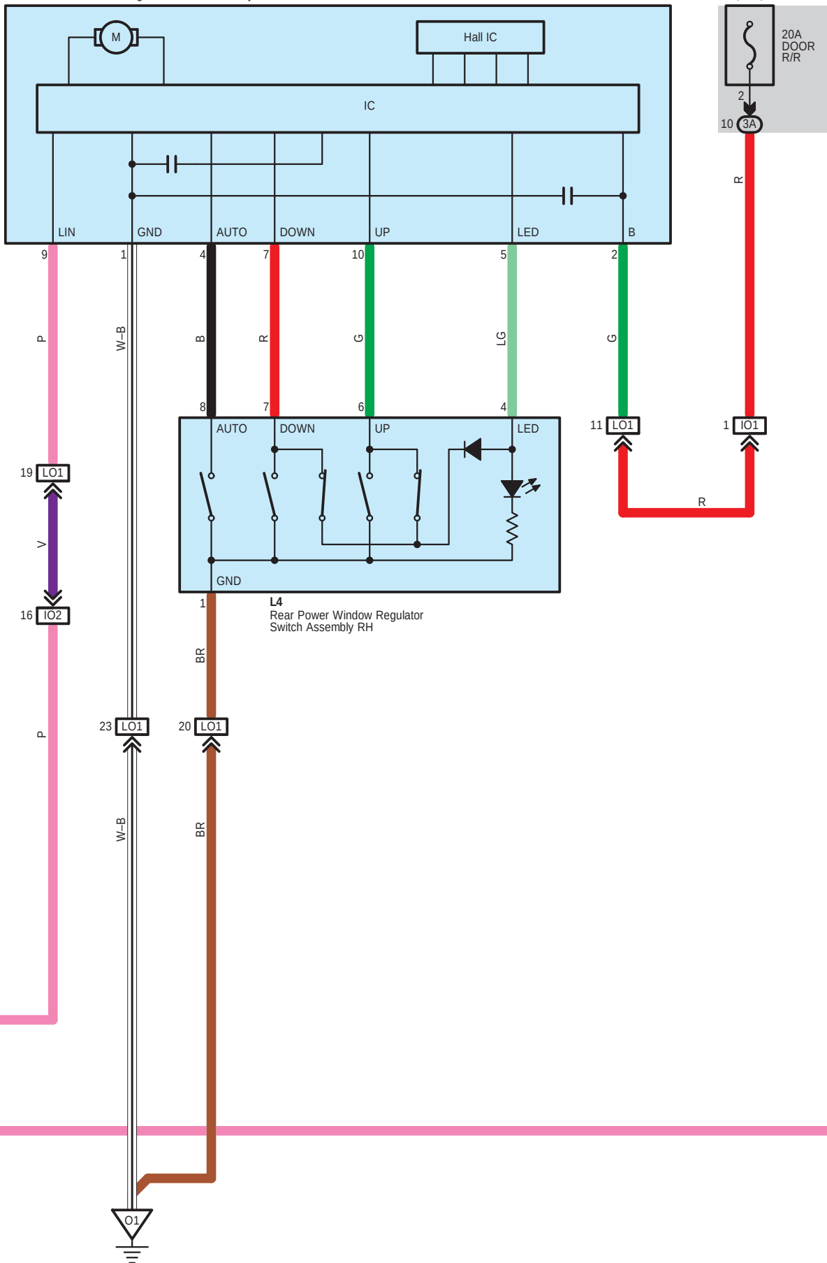
L2 Rear Power Window Regulator Motor Assembly RH
