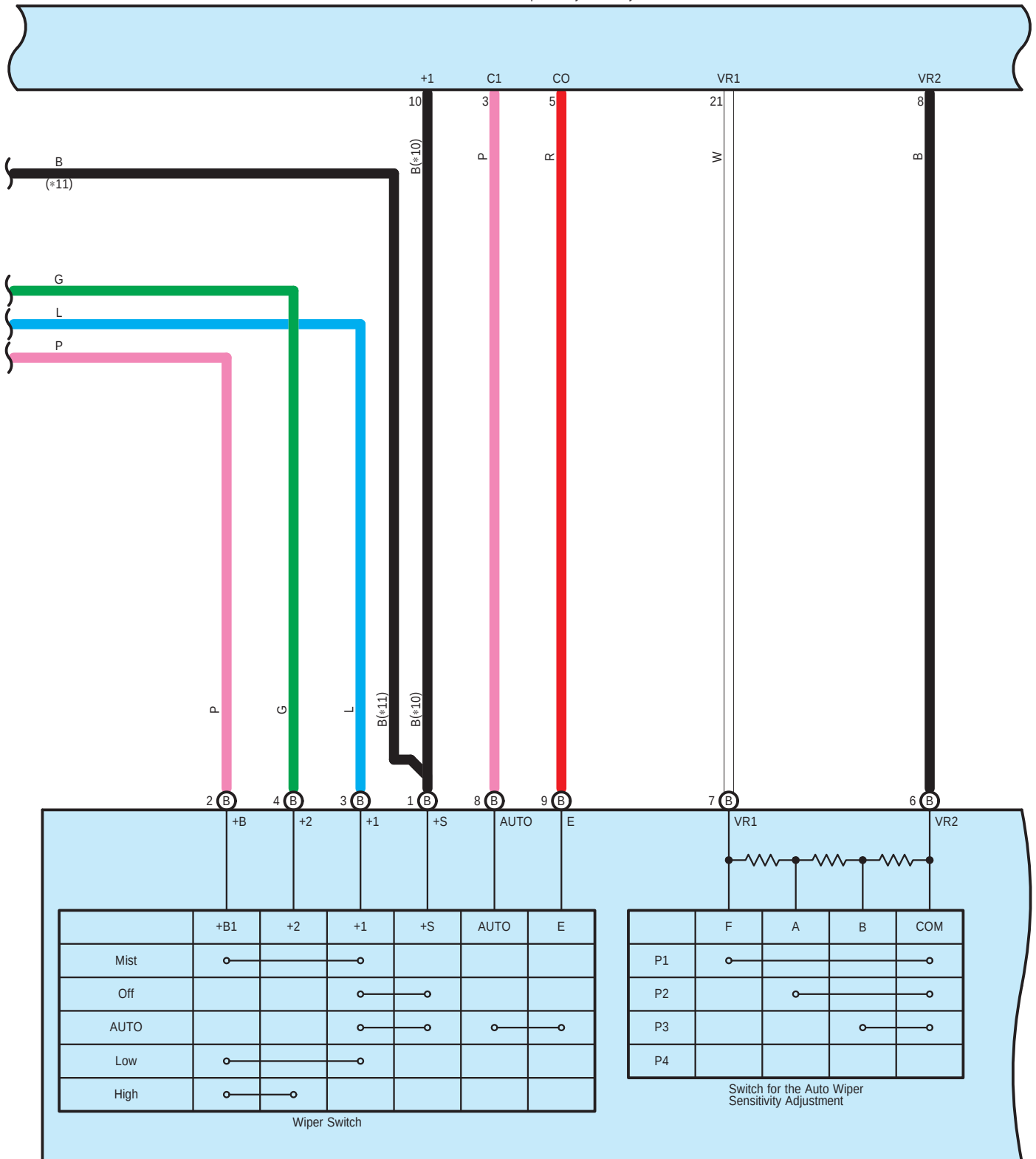
I31(A), I32(B) Windshield Wiper Switch Assembly
