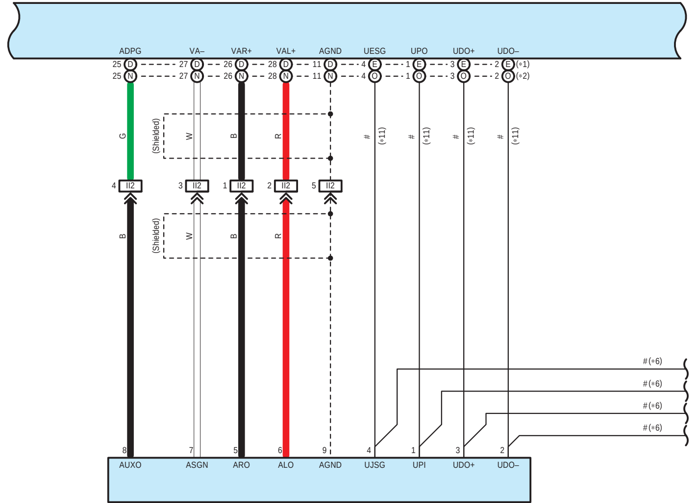
I146 No. 1 Stereo Jack Adapter Assembly
