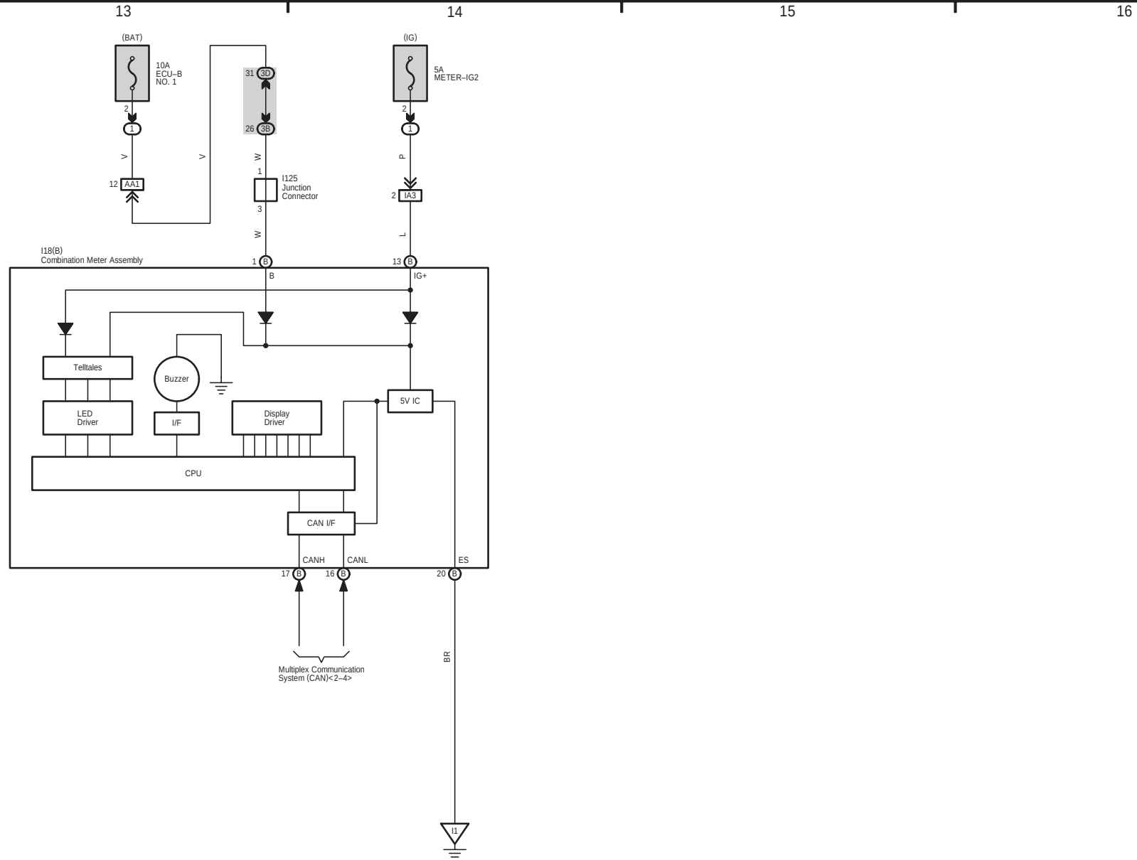
Hybrid Vehicle Immobiliser System, Smart Key System, Starting, Steering Lock and Wireless Door Lock Control
