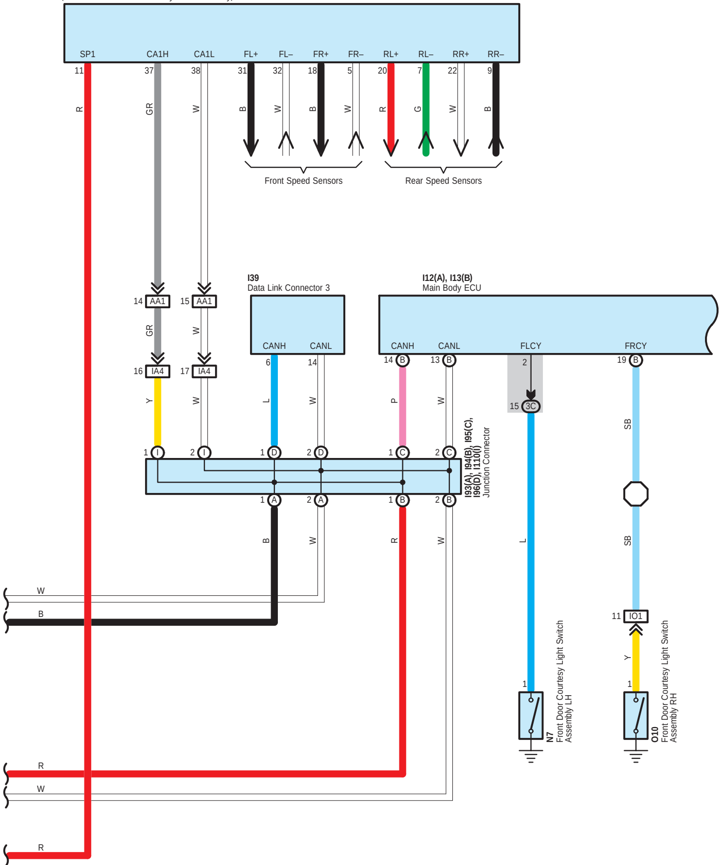
A28 Skid Control ECU with Actuator (Brake Booster with Master Cylinder Assembly)
