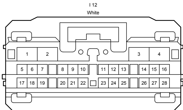
(Low LED Type, High LED Type and LED Daytime Running Light)
