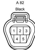
(Low LED Type, High LED Type and LED Daytime Running Light)
