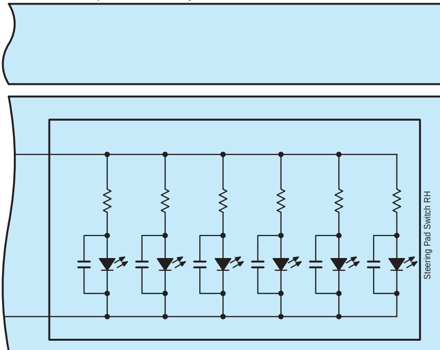
z3(E) Steering Pad Switch Assembly
