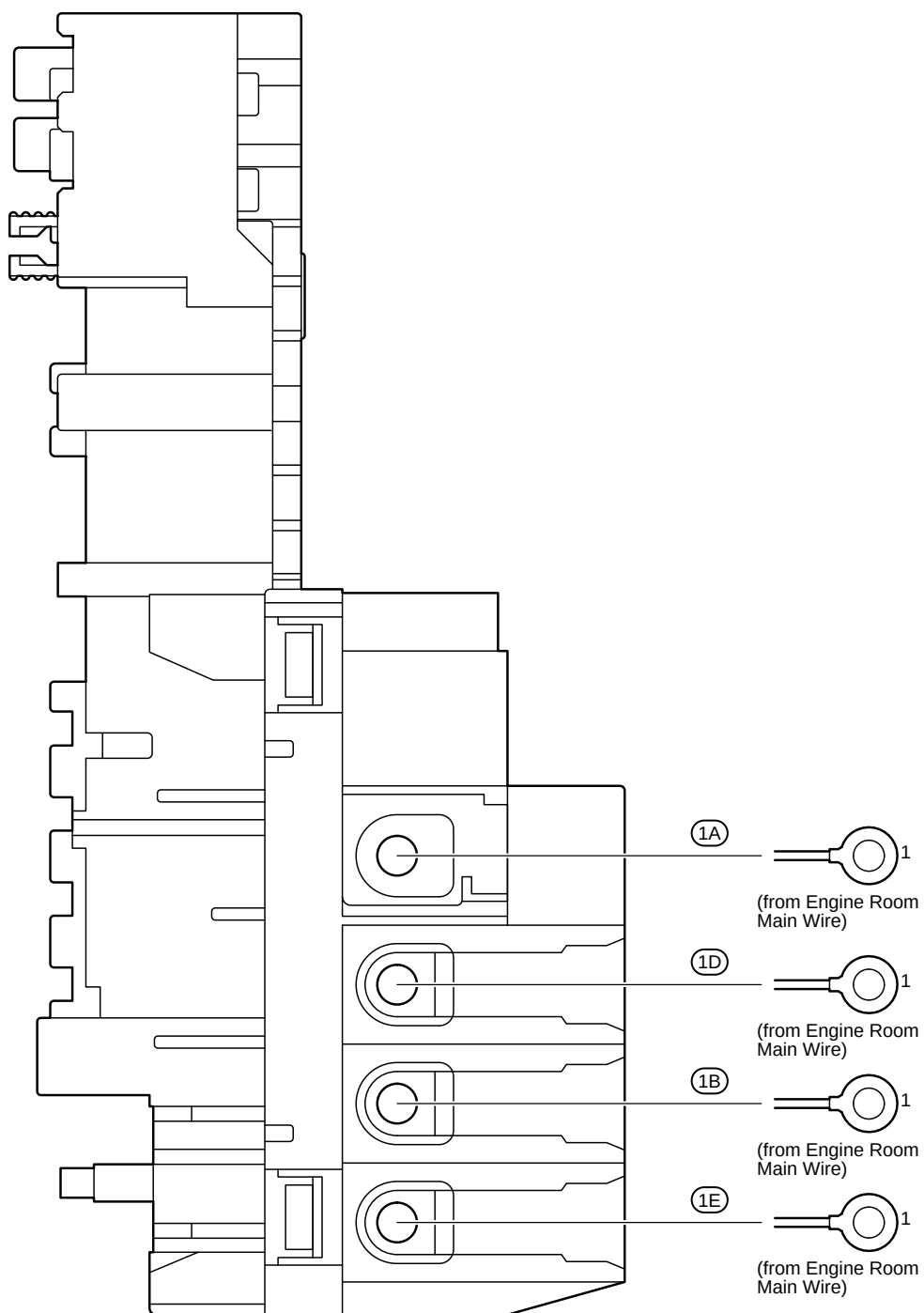
Side View
