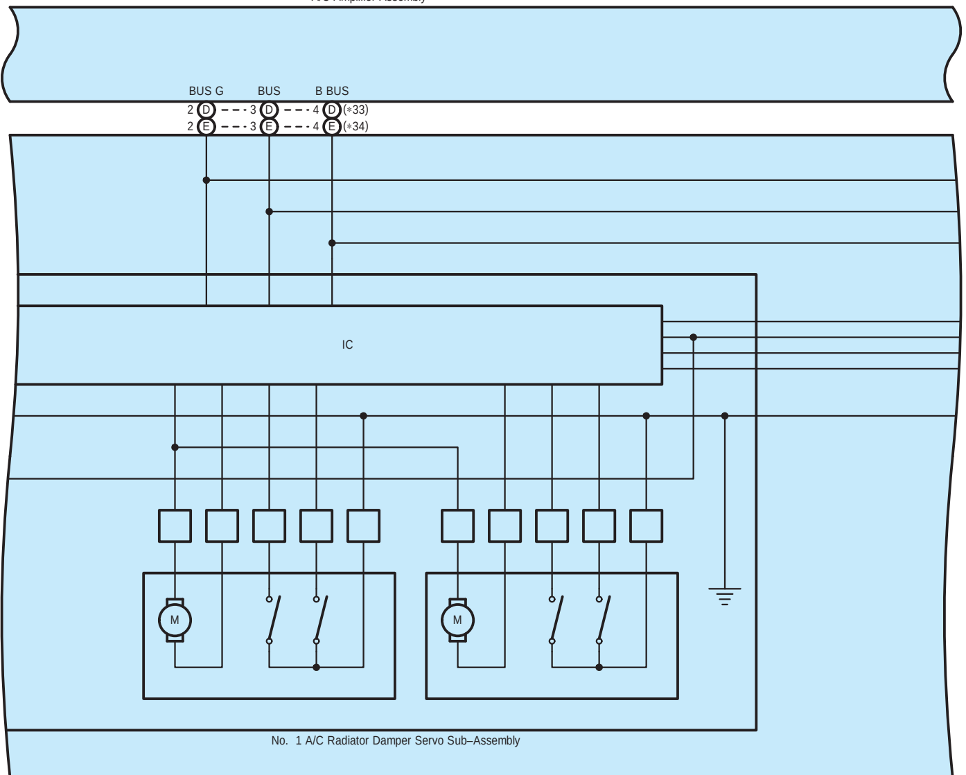
z8(D), z11(E) A/C Unit (A/C Harness Assembly)
