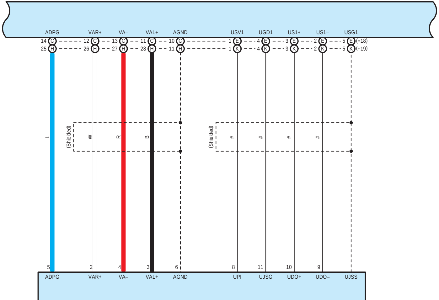
K5 Stereo Jack Adapter Assembly No. 1
