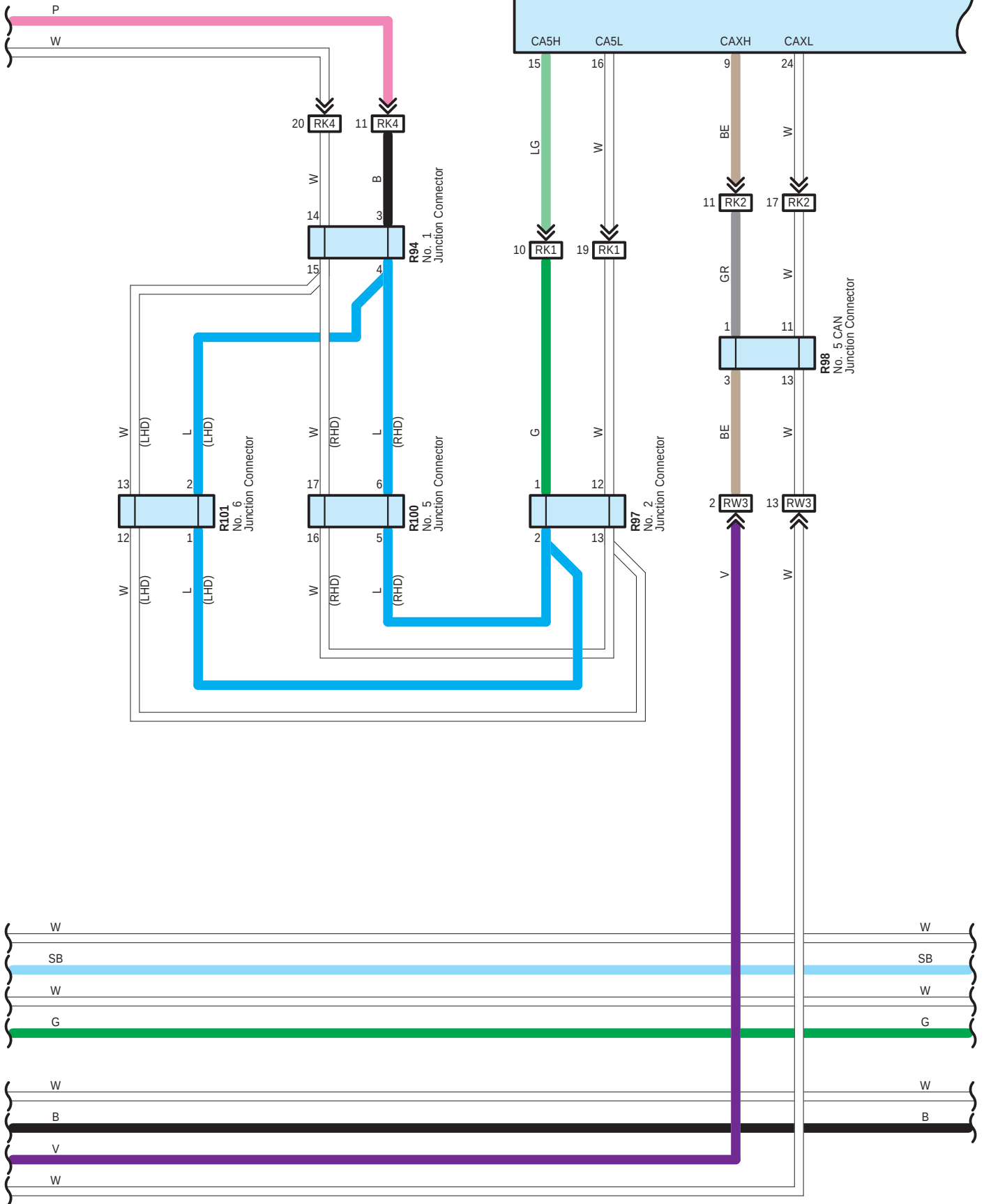
K76 Network Gateway ECU (Central Gateway ECU)
